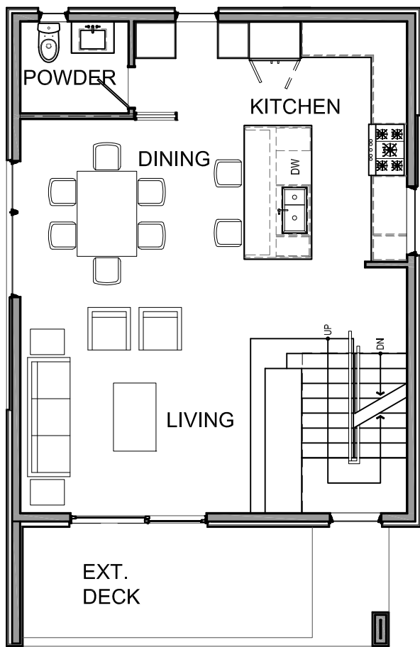
2ND FLOOR
